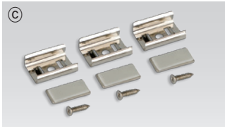
⑦ Mounting bracket : HDV-BRACKET1 Included in fixture
