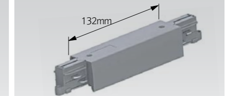
㉙ TRACK047-264 / FLEX 60 CONNECTER
