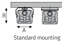
Standard mounting
