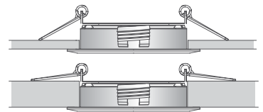
Mounting spring installation
