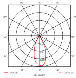
DVS4A 40K-24V-45
