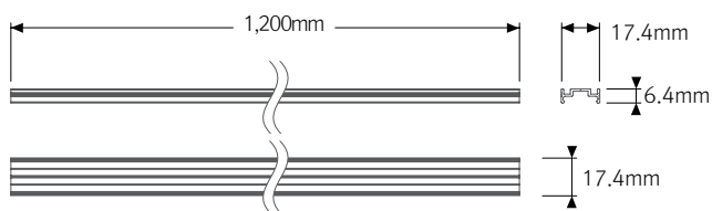
* MNR-Rail extrusion line
