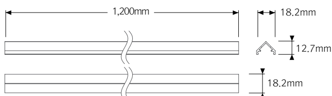
* MNR-Rail extrusion corner
