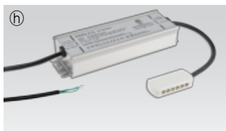
h LED Driver : FLC200-24V/T (200W 24V)
