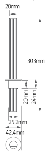
* MNR-Rail extrusion pole
