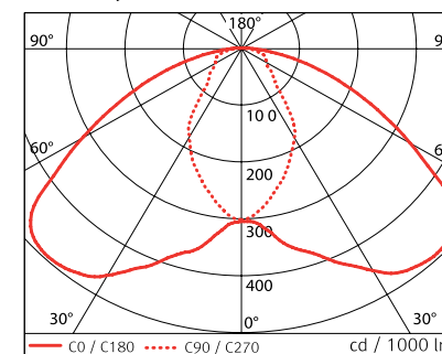
Polar Luminous Intensity Distribution
