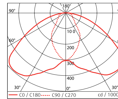
Polar Luminous Intensity Distribution
